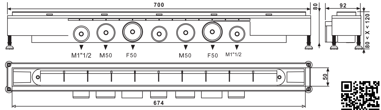
Plan / Drawing = mm
