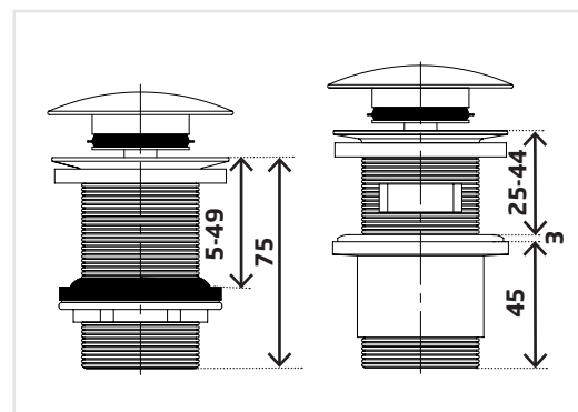
Rotative plug
