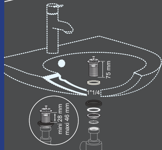
1.25" CHROMED BRASS WASTE WITH ANTI-VANDALISM PLUG for washbasin with built-in overflow.
