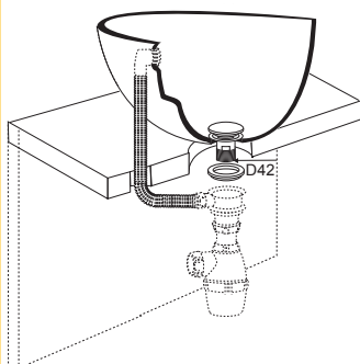
Basin with integrated overflow
